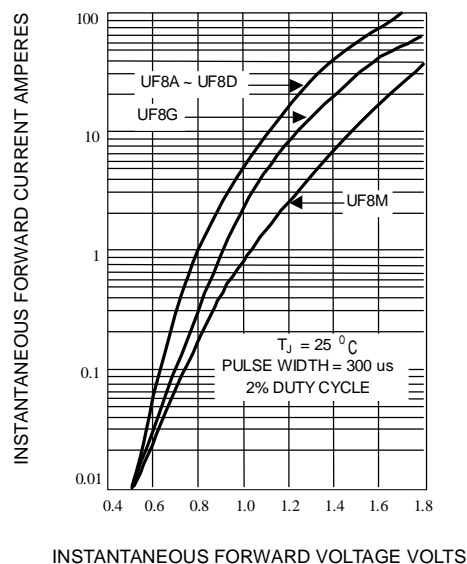
Fig. 4-TYPICAL FORWARD CHARACTERISTICS
